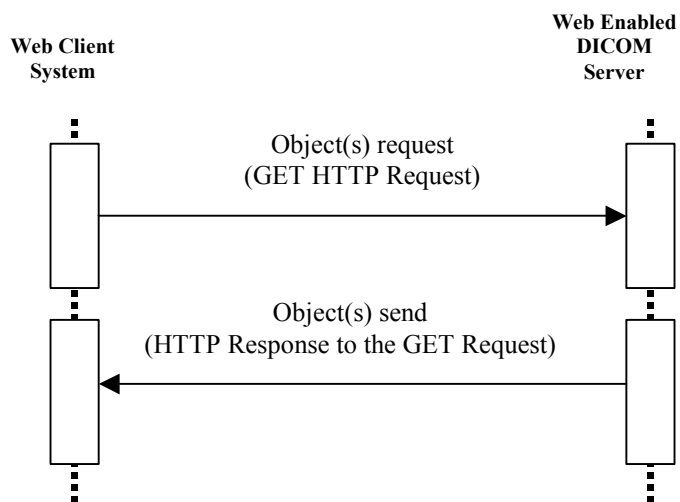
Figure 6-1 — Interaction Diagram
